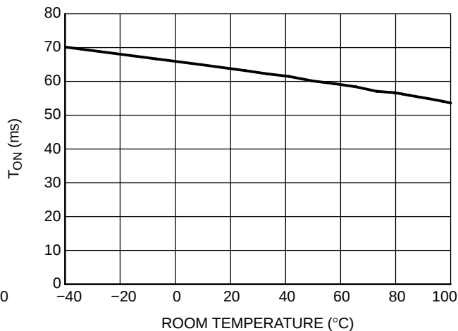
Figure 17. Turn On Time versus Room Temperature @ V_{BAT} = 3.6 V, C_{BYP} = 1 \mu F , C_{IN} = 100 nF, R_{IN} = 22 k, R_F = 110 k
