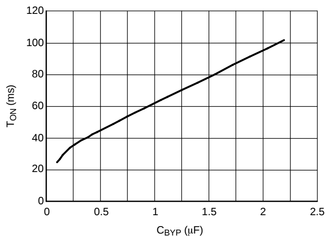
Figure 18. Turn On Time versus C_{BYP} @ V_{BAT} = 3.6 V, T_A = +25^\circ C , C_{IN} = 100 nF, R_{IN} = 22 k, R_F = 110 k
