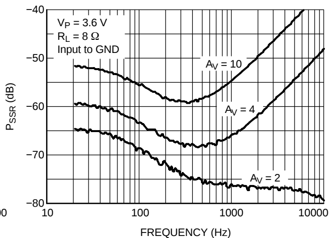
Figure 15. P_{SRR} versus Frequency and Gain @ V_P = 3.6 V
